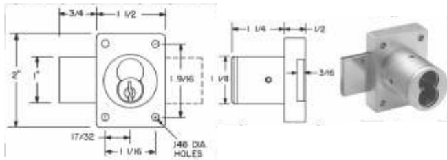
IC Core Cabinet Door Lock OL721DR-26D
