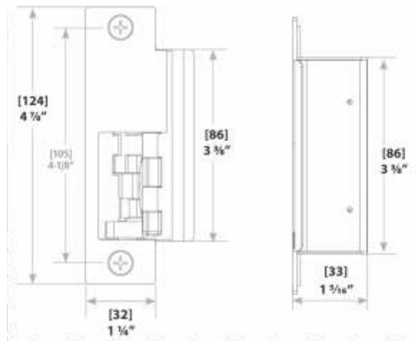
HE8500 Body only
