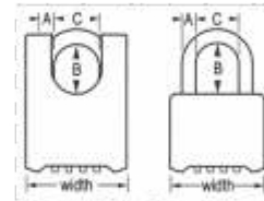
Shackle Dimensions
