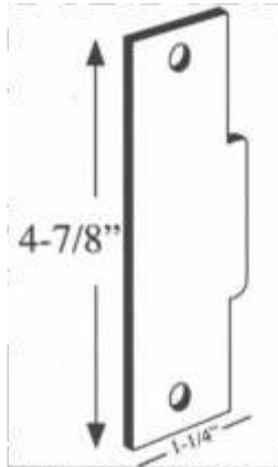
PLEFP-110 Filler Plate 4 7/8" x 1 1/4"
