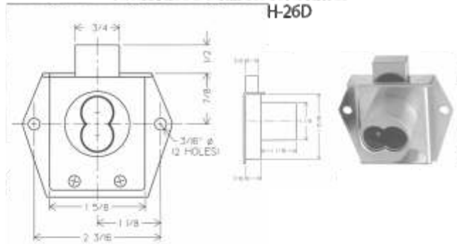
IC Rim Deadbolt VH Drawer 26D
