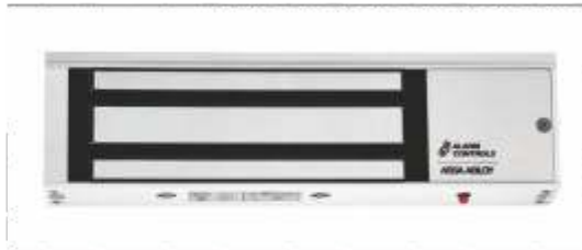
AC600LB 600 lbs Single Lock with Bond Sensor, Door Status Sensor and LED
