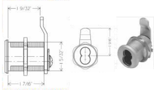
IC Cam Lock 1 1/4" L/Core OL720LM/DM-26D
