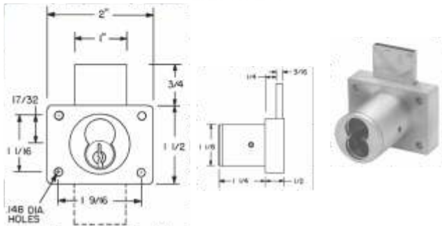
IC Core Cabinet Drawer Lock OL721DW-26D
