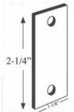
PLEFP-120 Filler Plate 2 1/4" x 1 1/8"
