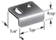
STRIKE PLATE 5/16" ANGLE TMC100SP-19
