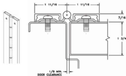
FS-302 FULL SURFACE FLUSH MOUNT
