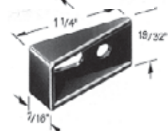
DRAWER CLIP TMC500DC-19
