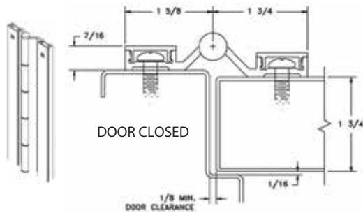
FS-101 FULL SURFACE 1/8" INSET
