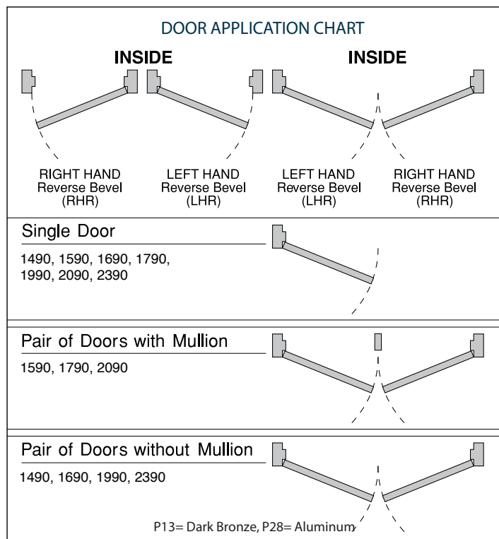
1990 Series Concealed Vertical Rod Device
