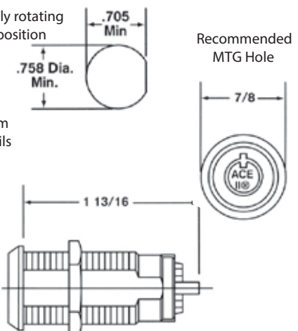
C4073 Dimensions
