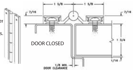
FS-102 FULL SURFACE FLUSH MOUNT
